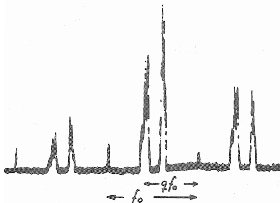
Fig. 1 - Frequency spectrum of the difference signal derived from two plates and induced by the Schottky noise in the beam. Small peaks harmonics of the revolution frequency. Large peaks fast and slow transverse waves.
