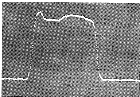
Fig. 3 - Scans of the longitudinal density in a stacked beam.
