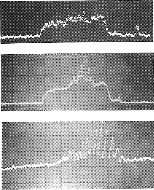
Fig. 5 - Transverse Schottky scan of the slow wave f = (43 - Q)f_0 showing amplitude growth due to 8th order and 11th order non-linear resonances.
