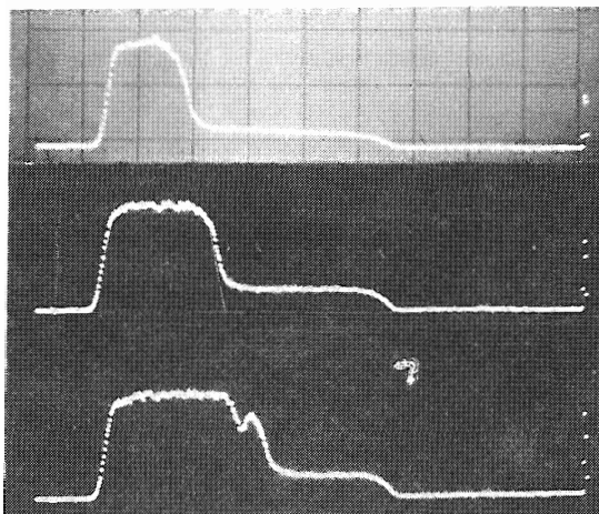
Fig. 2 - Longitudinal Schottky scan taken at different intensity levels during build-up of a stack (10 A, 15 A, 19 A). Average over \sim 2000 samples. \Delta p/p = 6.4\% per hor. Division.
