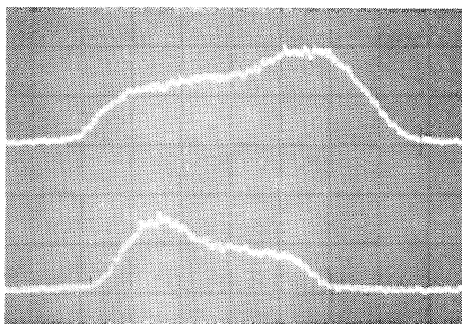
Fig. 4 - Transverse Schottky scan of a 6,5 A beam. Average over \sim 6000 samples. 2 kHz/hor. Division.
