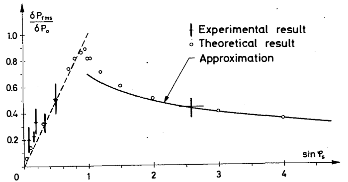
Fig. 1. Normalised r.m.s. momentum spread as function of \sin \phi_s .
