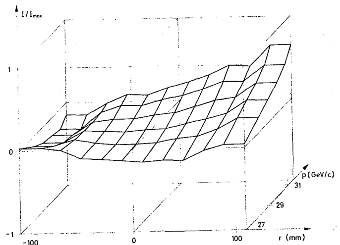
Fig. 3. Normalized currents in the pole-face windings of the focussing magnet units as function of radial position and momentum.
