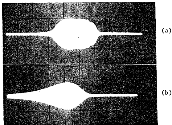
Fig. 5. Empty bucket signal induced on p.u. station (a) initial 11.9A stack at 26.5 GeV/c (b) 6A stack at 31 GeV/c after phase displacement
