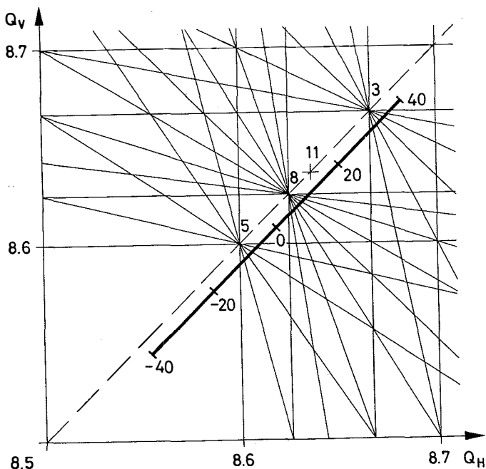
Fig. 2. The working line used for the phase displacement acceleration.
