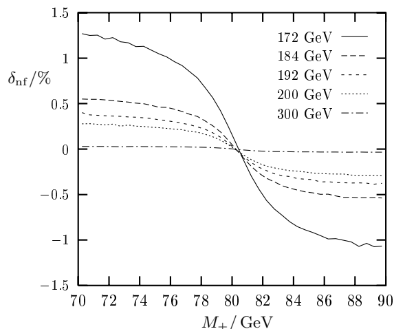
Fig. 1. Relative non-factorizable corrections to the invariant-mass distribution d\sigma/dM_+ in e^+e^- \rightarrow \mu^+\nu_\mu\tau^-\bar{\nu}_\tau for some CM energies (plot taken from Ref. [25]).
