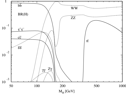
Fig. 1. Branching ratios of the SM Higgs boson as a function of its mass [10].
