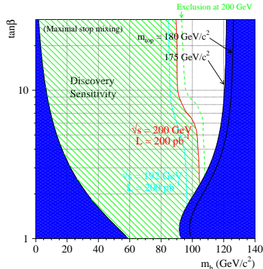
Figure 2: The sensitivity to MSSM Higgs bosons that may be achieved at LEP 2 [10].
