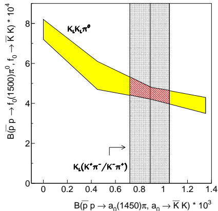
Figure 2: Determination of the branching ratio of f_0(1500) in the reaction \bar{p}p \rightarrow K_L K_L \pi^0 [4] (light hatched area), where it is correlated with the a_0(1450) production. The a_0(1450) contribution is fixed in the analysis of the reaction \bar{p}p \rightarrow K_L K^\pm \pi^m p [6].
