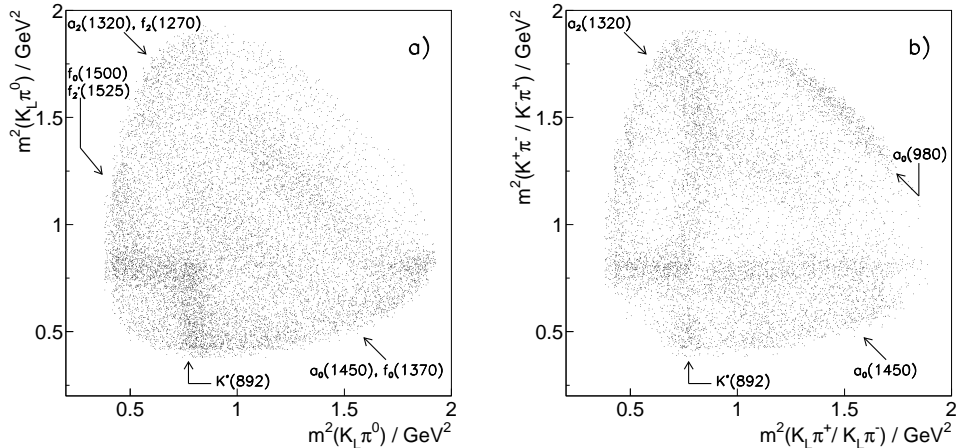
Figure 1: The Dalitz plots for the annihilation reactions a) \bar{p}p \rightarrow K_L K_L \pi^0 and b) \bar{p}p \rightarrow K_L K^\pm \pi^\mp p in liquid hydrogen.
